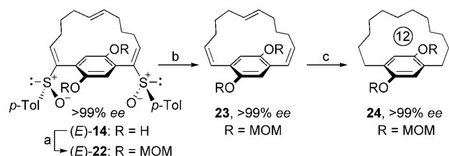
Scheme 8. Synthesis of 24 : a) MOMCl, i\text{Pr}_2\text{NEt} , \text{CH}_2\text{Cl}_2 , 40^\circ\text{C} , 5 h, 92%; b) t\text{BuLi} , toluene, -78^\circ\text{C} , 5 min, 75%; c) \text{H}_2 , 10% Pd/C, MeOH, room temperature, 1 h, quantitative.
